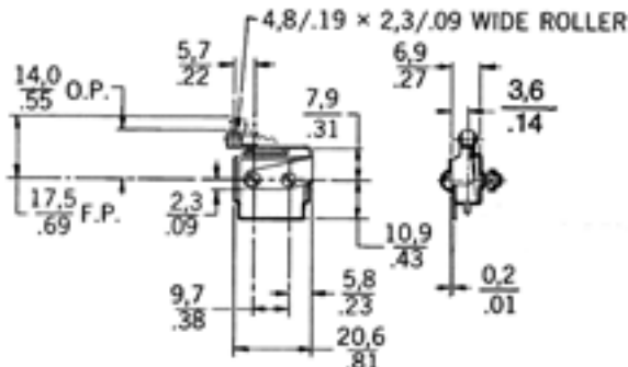
Figure 7. JS-308 Dimensions
